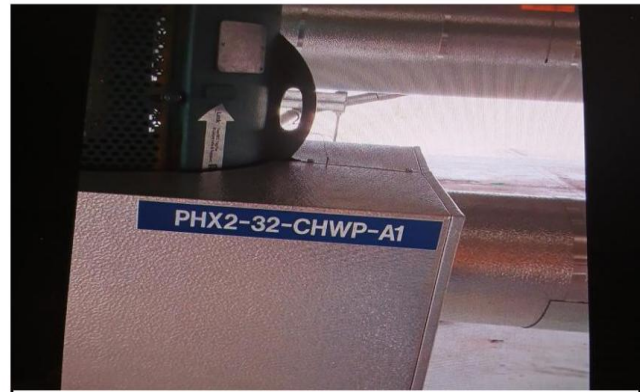
Follett, 500 hp Horizontal chiller pump in running backwards with 14 psi suction energy See Video
