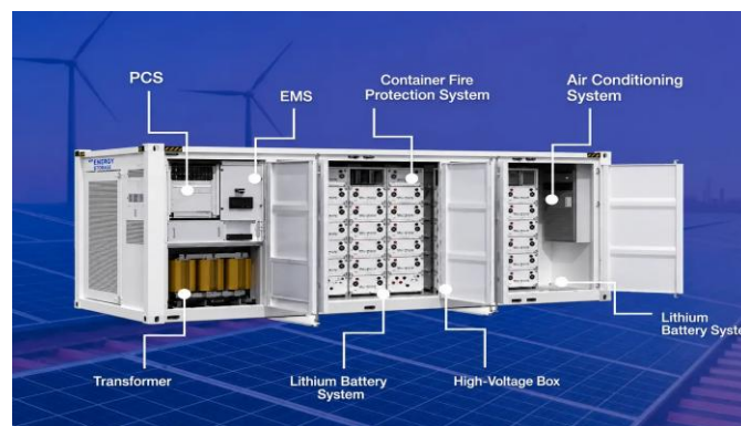
Kunetic container BESS with six subsystems.
